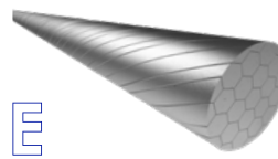
31 strands slick - Medium flexible, extra smooth
